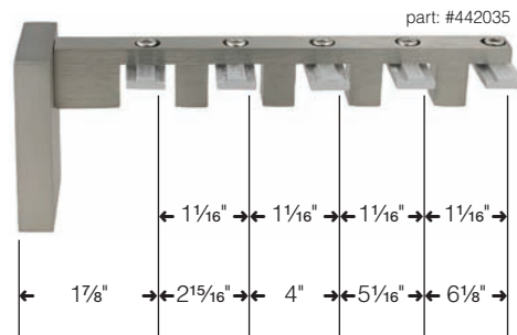
Side Bracket *4-panel sample - SN finish
