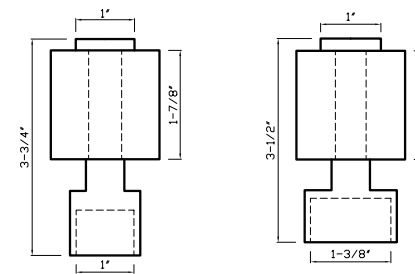
KS007 A Fits 1" Rod
