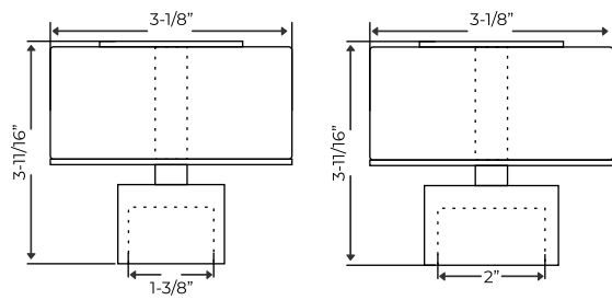
DC - 2040 B Fits 1 - 3/8" Rod
