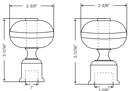
DC-2044 A Fits 1" Rod
