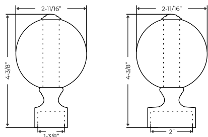
DC-2042 B Fits 1 - 3/8" Rod
