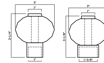
KS011 FITS 1" ROD
