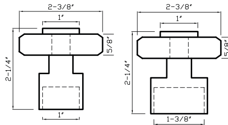
KS012 A Fits 1" Rod
