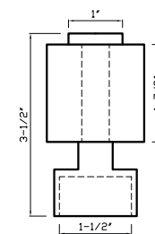
KS017 Fits 1 - 1/2" Rod
