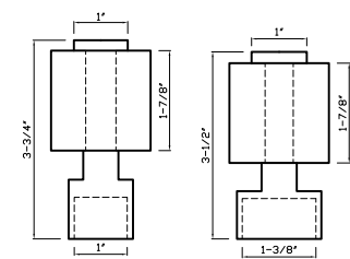
KS007 FITS 1" ROD
