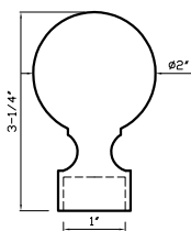
DC103 A FITS 1" ROD
